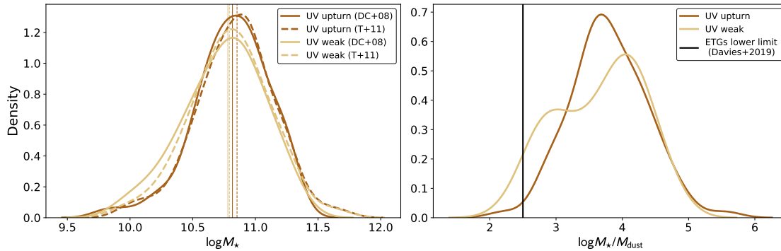
Figure 5.3: The left panel displays the comparison between the distributions of \log M_\star retrieved from MAGPHYS (da Cunha, Charlot, & Elbaz, 2008) and the estimates of Taylor et al. (2011, with the medians represented by the corresponding dashed lines) – which have been previously used in Chapters 3 and 4 – for UV weak and upturn systems. This image aims at showing that both distributions are in good agreement before exploring mass ratios exclusively retrieved from da Cunha, Charlot, and Elbaz (2008). The right panel displays the distribution of \log M_\star/M_{\text{dust}} for MAGPHYS; the black straight line is the threshold of 2.5 established by Davies et al. (2019a).
