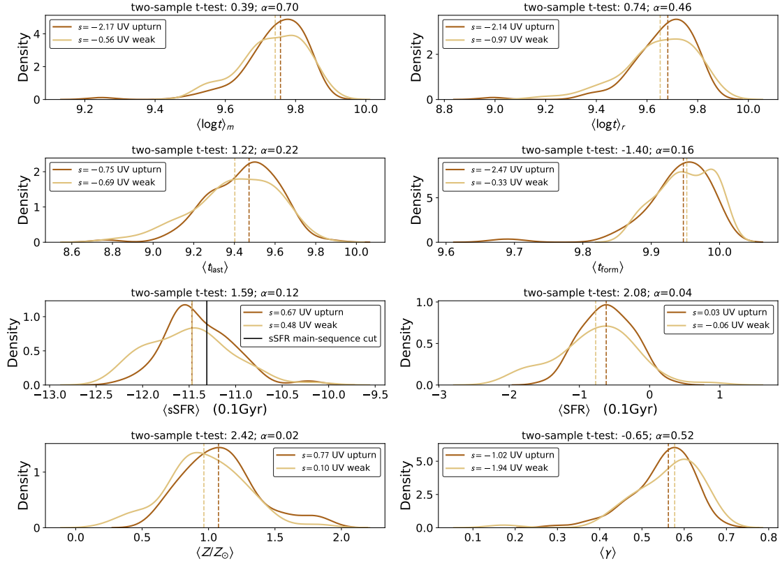
Figure 5.5: Distributions of several parameters which resulted from SED fitting by MAGPHYS (da Cunha, Charlot, & Elbaz, 2008). Left panel (from top to bottom): mass-weighted median stellar age ( \langle \log t \rangle_m ); median time since last burst of star-formation ( \langle t_{\text{last}} \rangle ); median specific star-formation over the past 0.1 Gyr ( \langle \text{sSFR} \rangle ); median metallicity ( \langle Z/Z_{\odot} \rangle ). Right panel (from top do bottom): light-weighted (based on the r -band) median stellar age ( \langle \log t \rangle_r ); median age of the oldest stars in the galaxy ( \langle t_{\text{form}} \rangle ); median star-formation rate over the past 0.1 Gyr ( \langle \text{SFR} \rangle ); median star-formation timescale ( \langle \gamma \rangle ). The median values for each distribution is displayed in dashed lines, except for \langle \text{sSFR} \rangle , which the medians are exactly the same; therefore, the median of UV upturn systems is displayed in a continuous line to allow the reader to see the overlapped values. Also, the star-formation main sequence cut is displayed via a black straight line for \langle \text{sSFR} \rangle at -11.31 (see, for instance, Davies et al., 2019b). A two-sample t-test and p-value are displayed at the top of each subfigure.
