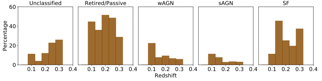
Figure 4.3: Bar-plots similar to those of Fig. 3.2 stratified by WHAN classes.
