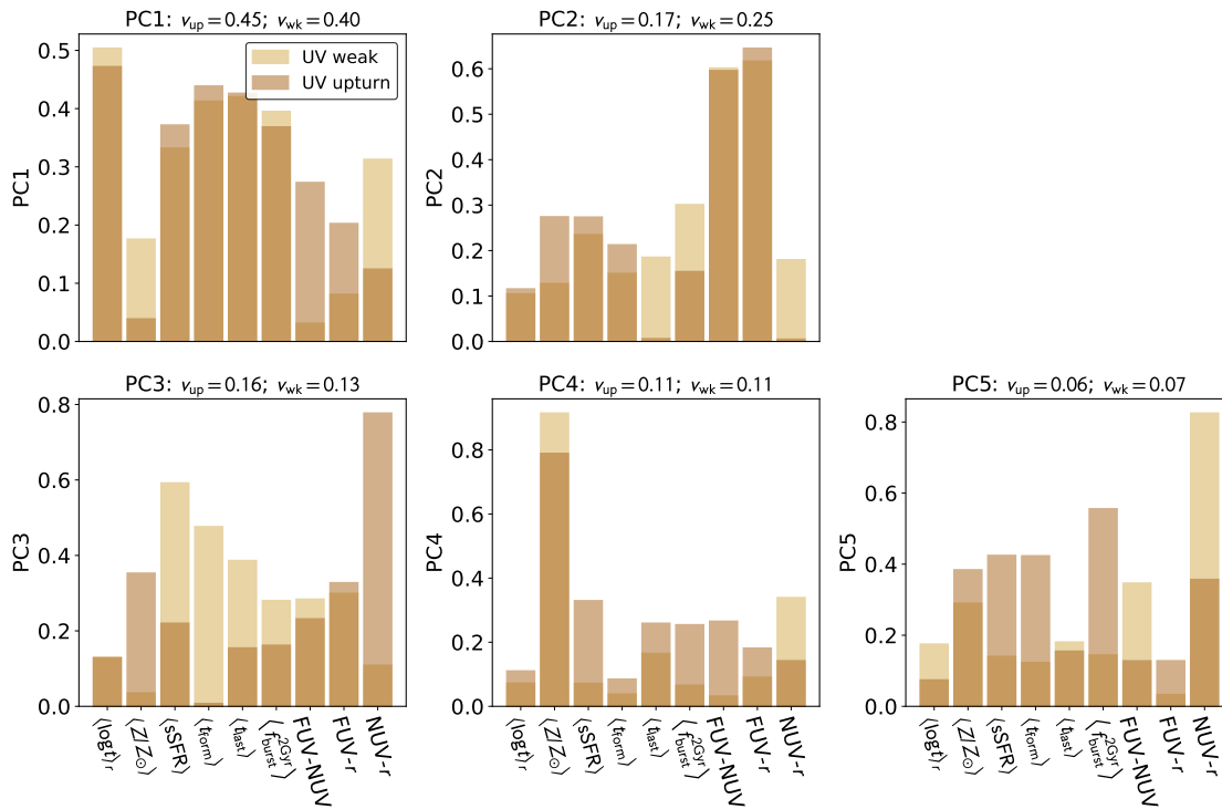
Figure 5.10: Principal components (PCs) resulting from the PCA technique. The results depict UV weak and UV upturn systems in light and dark brown respectively. The contributions to the total variance are available in the respective titles of the sub-plots (i.e. v_{wk} for UV weak and v_{up} for UV upturn galaxies).
